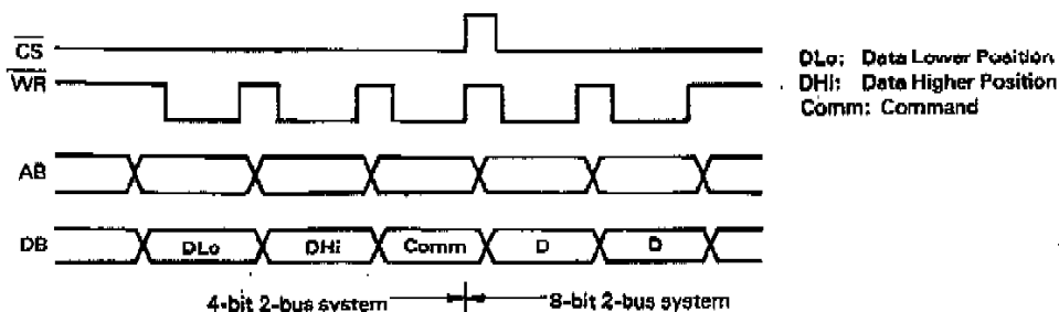
Fig. 3.6-3 Example of Data Transfer Mode Change
