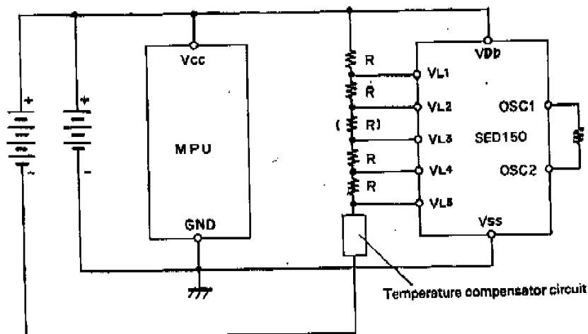
Fig. 3.3-1 Basic Connection Diagram
