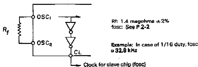
Fig. 3.5-3 CR Oscillator
