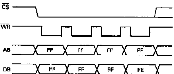
Fig. 3.6-3 Example of Data Transfer Mode Change
