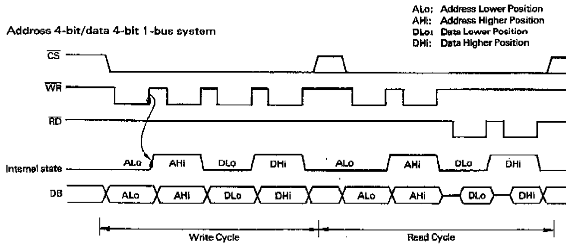
Fig. 3.6-1 Timing Sequence Examples
